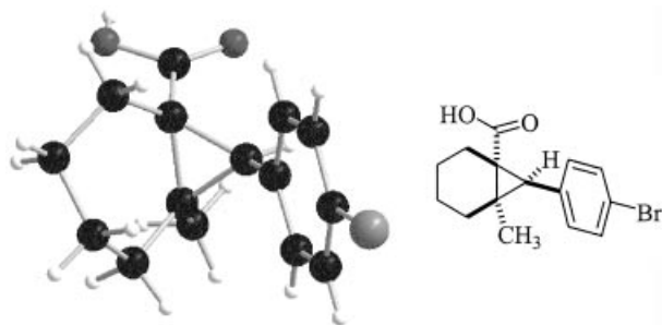
Figure 2. Solid-state structure of (1 R *,6 S *,7 R *)-6-(4-bromophenyl)-5-methylbicyclo[4.1.0]heptane-1-carboxylic acid ( rac - 13d ).
