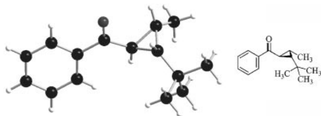
Figure 1. Solid-state structure of (1 S ,2 R ,3 R )-1-(2- tert -butyl-3-methylcyclopropyl)-1-phenylmethanone ( 5h ).
